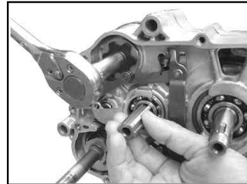
Close-ratio 6-speed • Set the stopper plate with the convex portion in the center to face outward.
