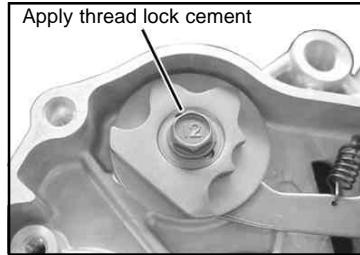
Close-ratio 4-speed • Set the stopper plate with the concave portion in the center to face outward.
