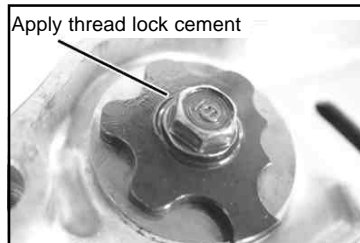
Close-ratio 6-speed • Set the stopper plate with the convex portion in the center to face outward.
