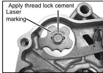
Close-ratio 5-speed
