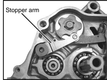
Close-ratio 4-speed • Set the stopper plate with the concave portion in the center to face outward.
